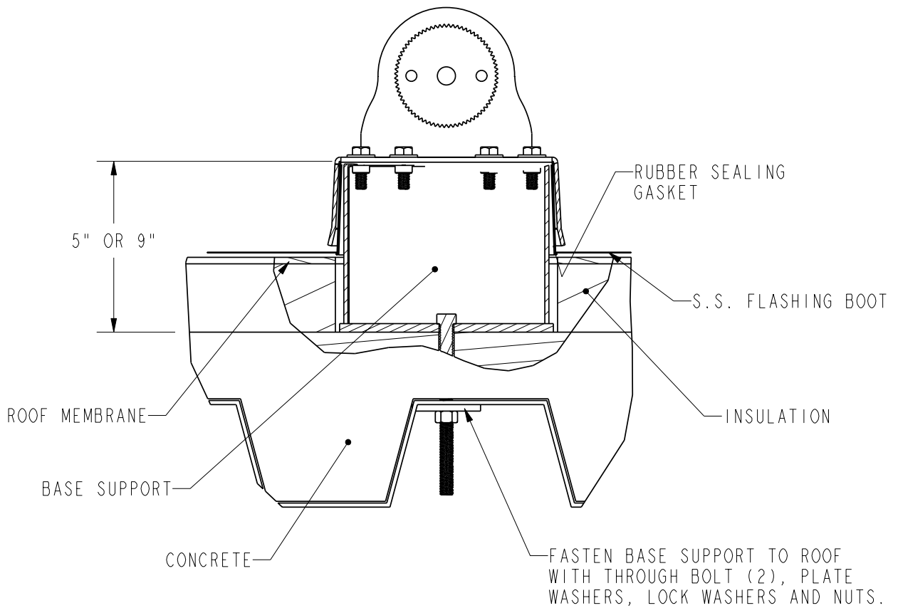
SECTION C-C
