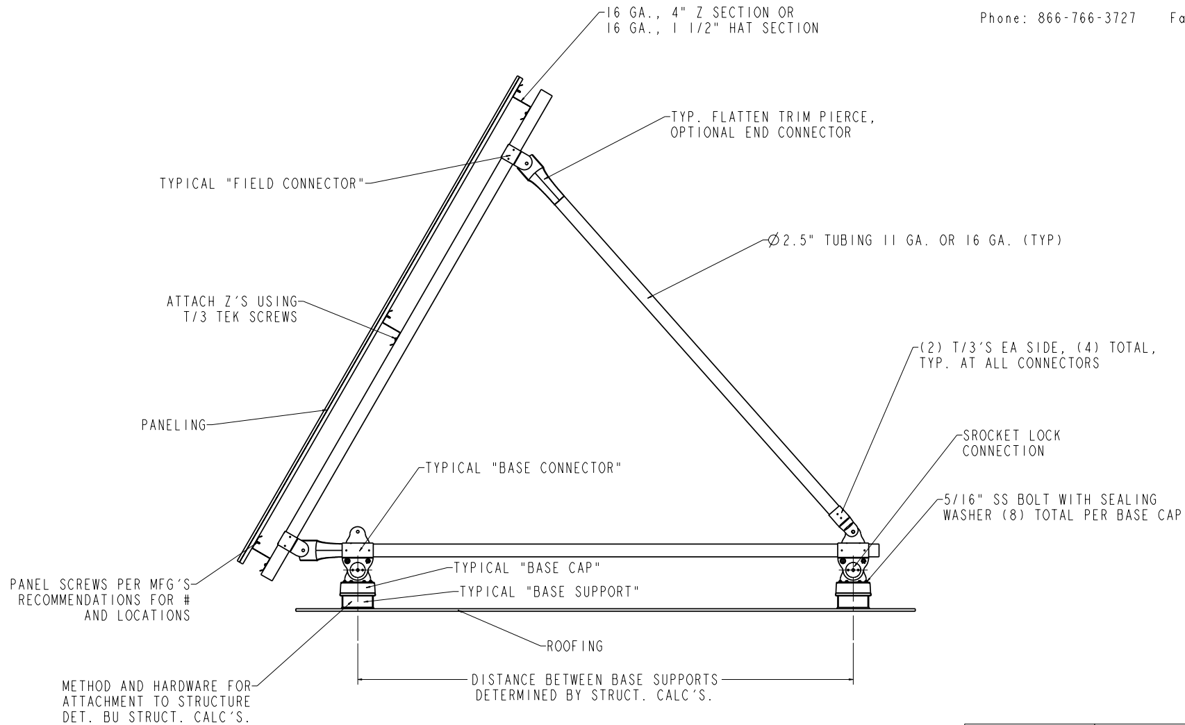
TYPICAL ROOFSCREEN TILTBACK FRAME
