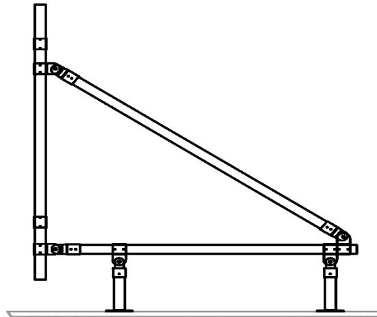
Example of RoofScreen SC3R Frame Configuration
