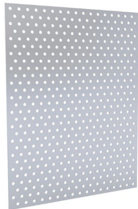
23% Open Area 1/8" hole @ 1/4" stagger
