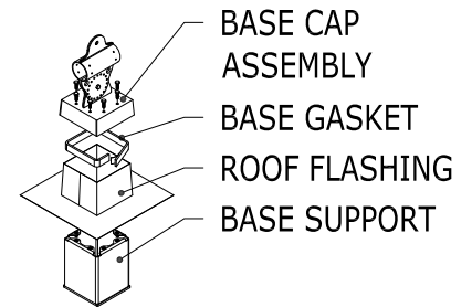
EXPLODED VIEW
