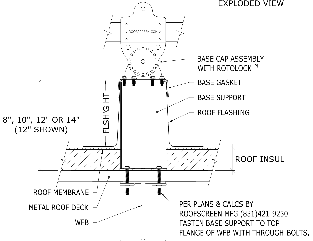
EXPLODED VIEW
