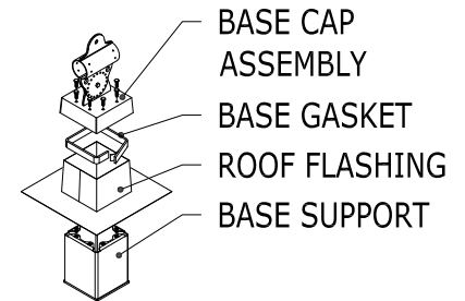
EXPLODED VIEW
