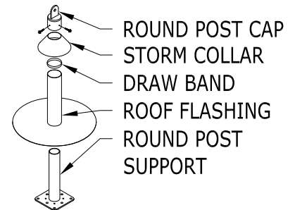
EXPLODED VIEW
