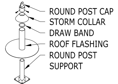
EXPLODED VIEW
