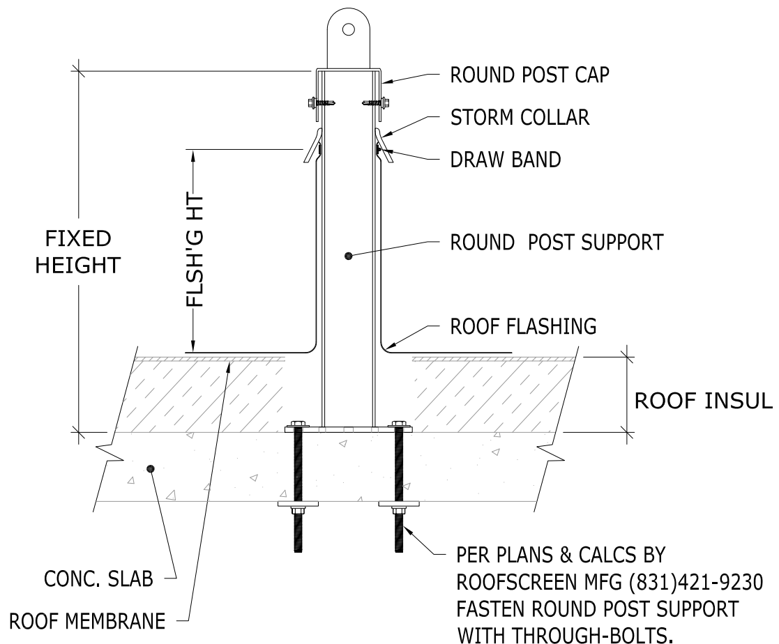
STRUCTURAL CONCRETE THROUGH BOLTS - WITH INSULATION
