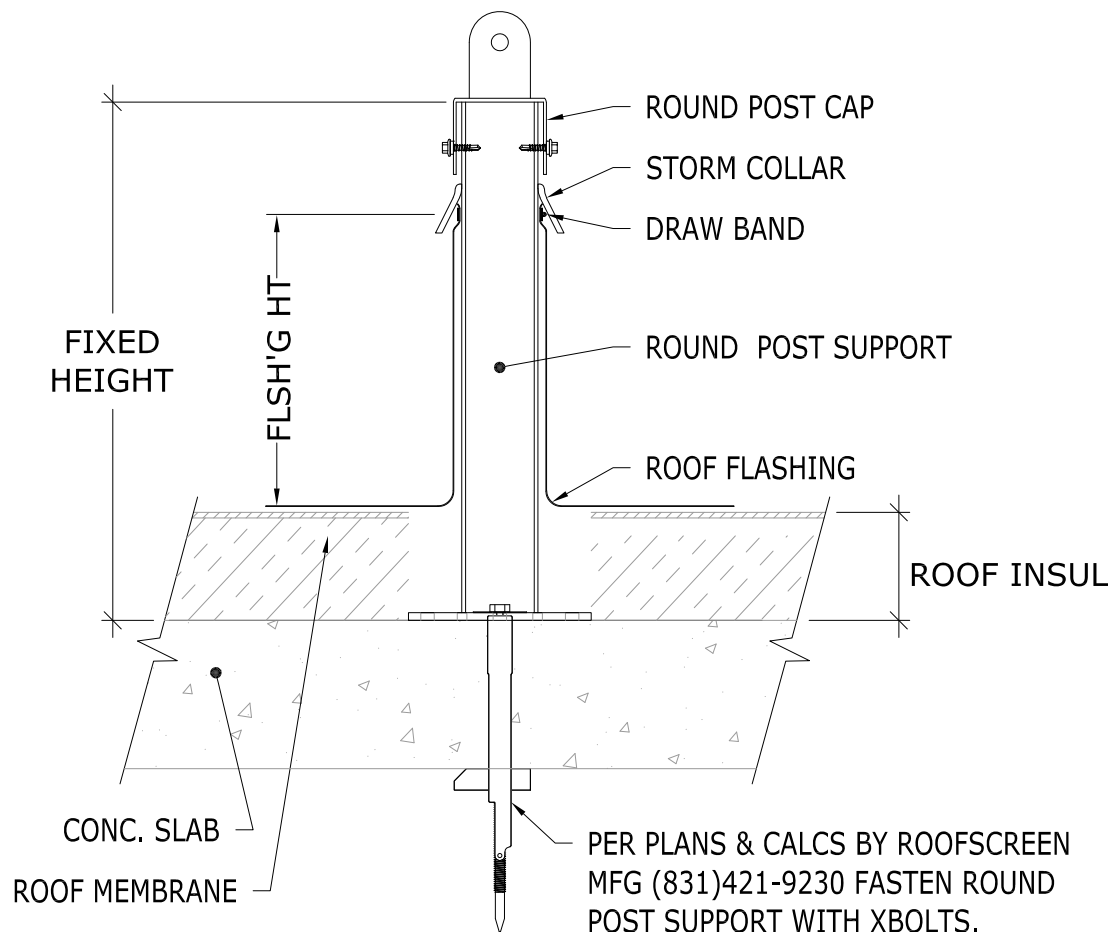
STRUCTURAL CONCRETE XBOLTS - WITH INSULATION
