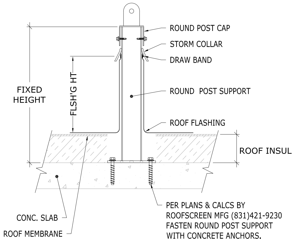
STRUCTURAL CONCRETE CONCRETE ANCHORS - WITH INSULATION
